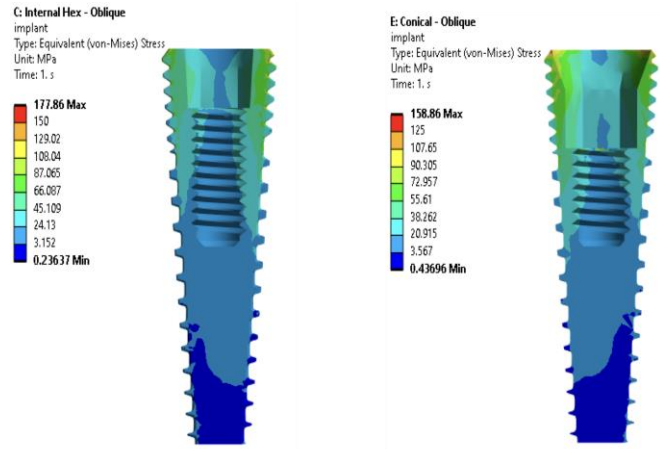
Figure 9: Stress distribution pattern on Implant of Internal Hex and Conical Hex Implant Abutment Connections under oblique load of 100N.
